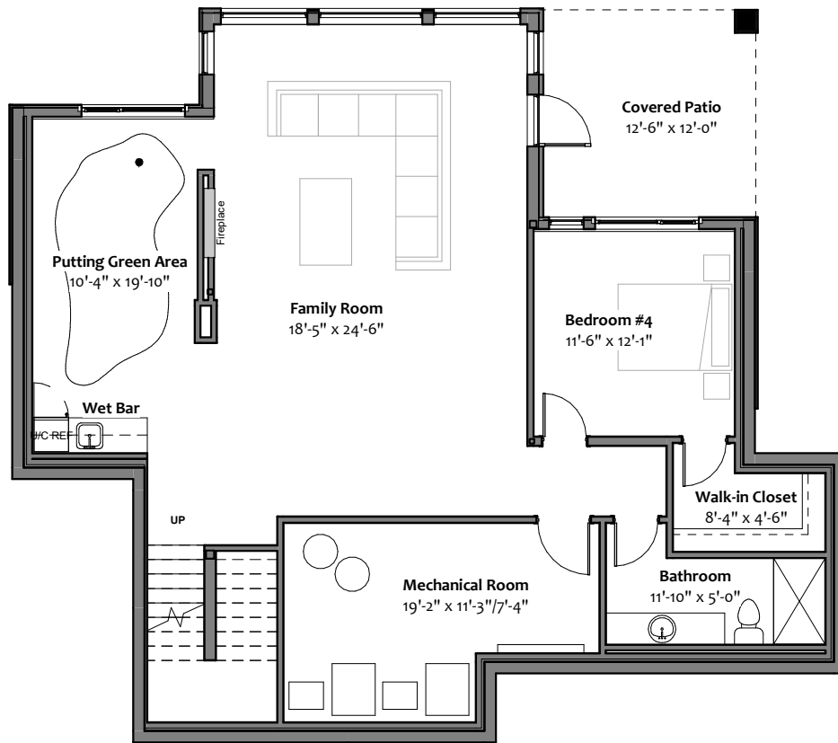
Basement Floor Plan 1426 ft 2
