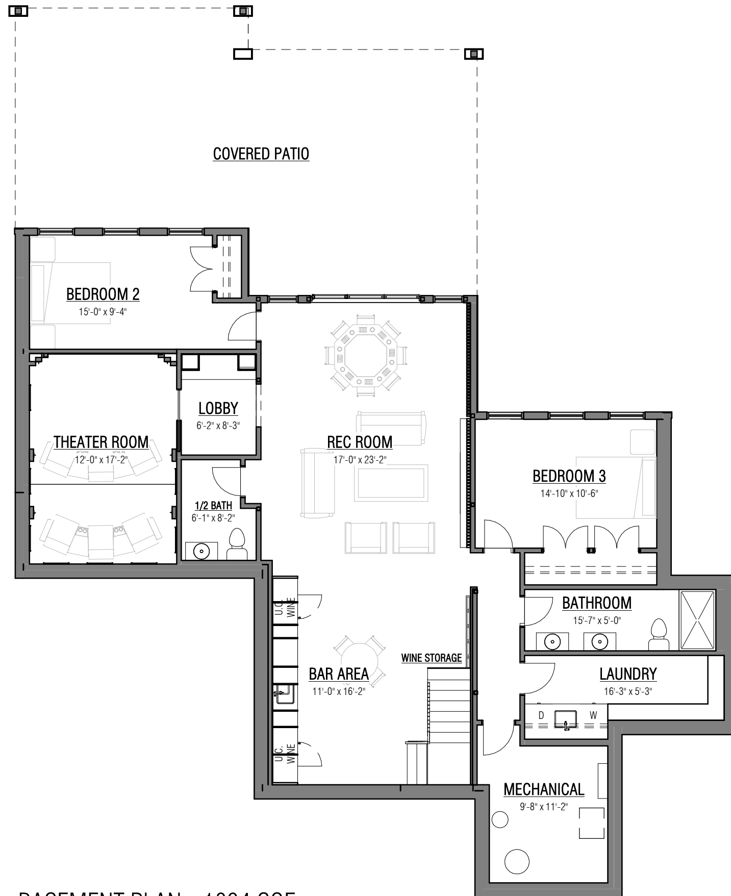
BASEMENT PLAN - 1804 SQF
