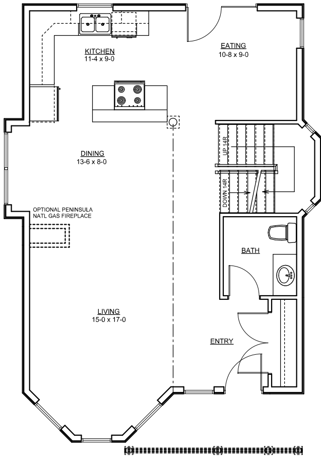
MAIN FLOOR PLAN 791 SQ FT
